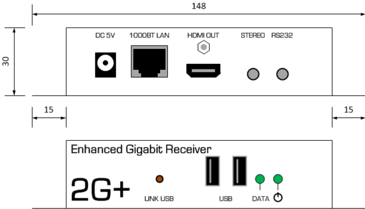
218A Front/Back
